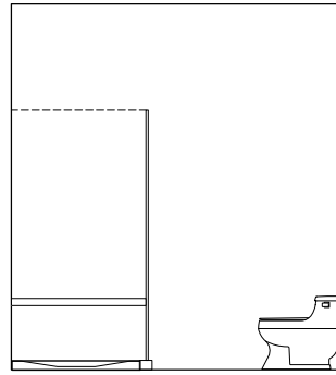
3 MASTER BATH ELEVATION
