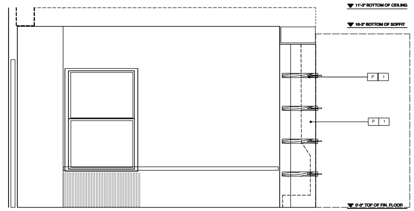
4 OFFICE ELEVATION
