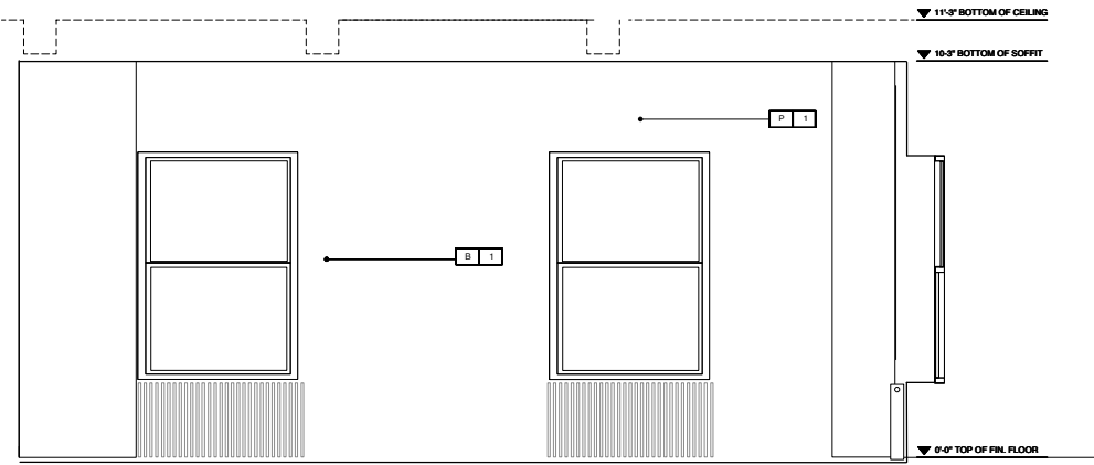
7 CONFERENCE ROOM ELEVATION
