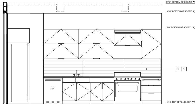
3 KITCHEN ELEVATION
