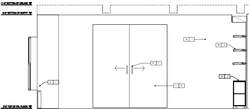
5 CONFERENCE ROOM ELEVATION
