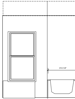
3 MASTER BATH ELEVATION
