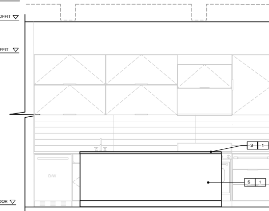
3 KITCHEN ELEVATION
