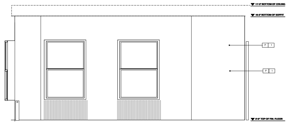
8 CONFERENCE ROOM ELEVATION
