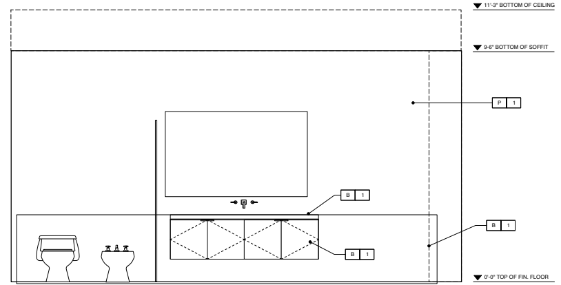
3 MASTER BATH ELEVATION
