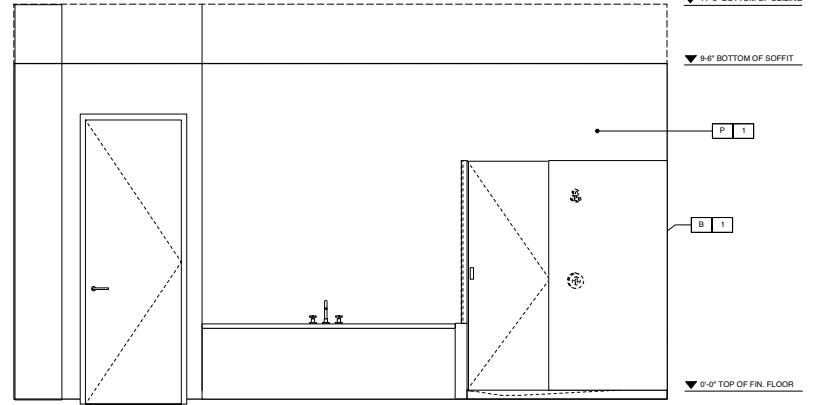
4 MASTER BATH ELEVATION
