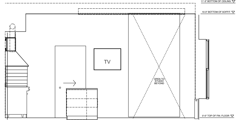
3 KITCHEN ELEVATION
