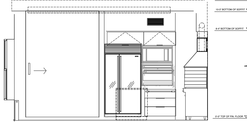
3 KITCHEN ELEVATION
